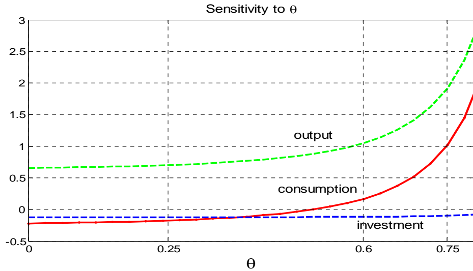
Figure 6. Impact Multipliers: Sensitivity to Non-Policy Parameters ( \theta, \varphi, \eta )
